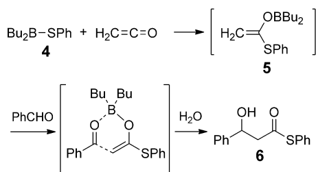
Scheme 7. The first example of a boron-mediated aldol reaction to give the \beta -hydroxy thioester 6 via the boron enolate 5 , which is generated from the thioester 4 and a ketene (Mukaiyama, 1973).
