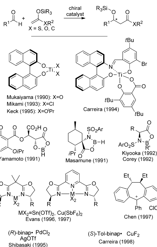
Figure 8. Chiral catalysts for catalytic enantioselective Mukaiyama aldol reaction (1990–1998). binap = 2,2'-bis(diphenylphosphanyl)-1,1'-binaphthyl.
