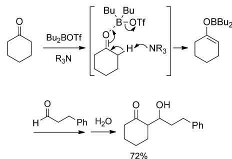
Scheme 8. Mukaiyama's original method for the generation of boron enolates from ketones using boron triflates and amines, with successive aldol reaction (1976).
