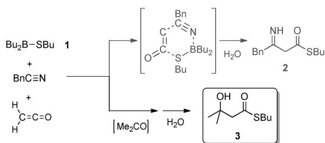
Scheme 6. Unexpected formation of the \beta -hydroxyalkanothioate 3 by a reaction of a ketene, the thioester 1 , and acetone (Mukaiyama, 1971).
